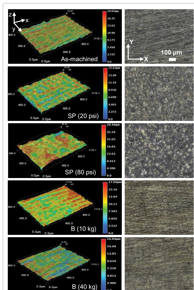
Figure 6: Surface topography maps of MgCa after shot peening at 20 and 80 psi and burnishing at 10 and 40 kg.
