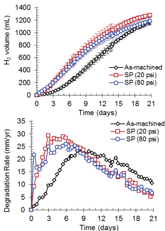
Figure 9: Hydrogen evolution and degradation rate of MgCa for 21 days in Hank's solution after shot peening (20 and 80 psi).
