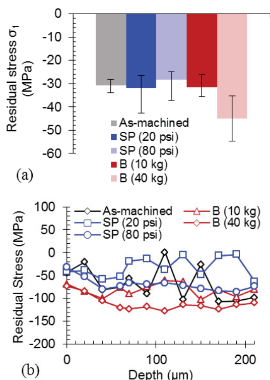
Figure 8: Residual stress in MgCa pins after shot peening at 20 and 80 psi and burnishing at 10 kg and 40 kg (a) on the surface and (b) along the depth (Co-K \alpha , 2\theta=141^\circ , 20 kV, 4 mA).
