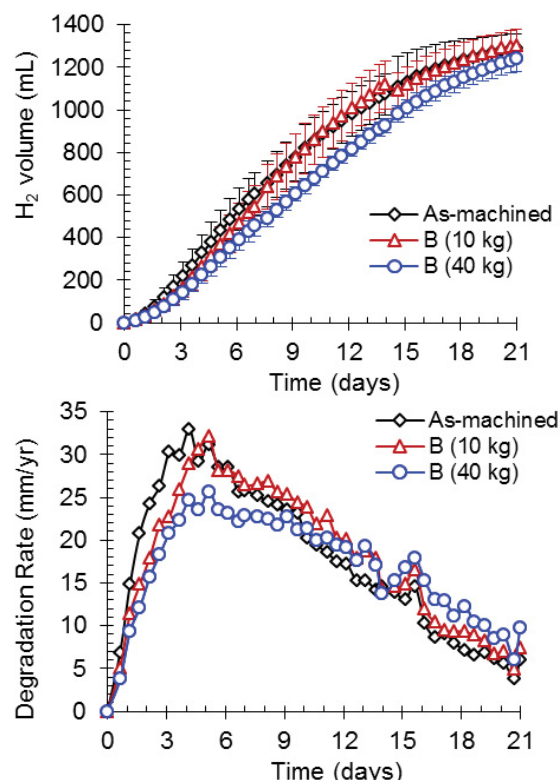
Figure 10: Hydrogen evolution and degradation rate of MgCa in Hank's solution for 21 days after burnishing (10 and 40 kg).
