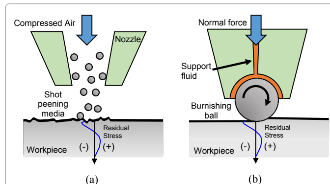
Figure 2: Process schematics of (a) shot peening and (b) burnishing to impart a favorable surface integrity that can influence stress-corrosion behavior.
