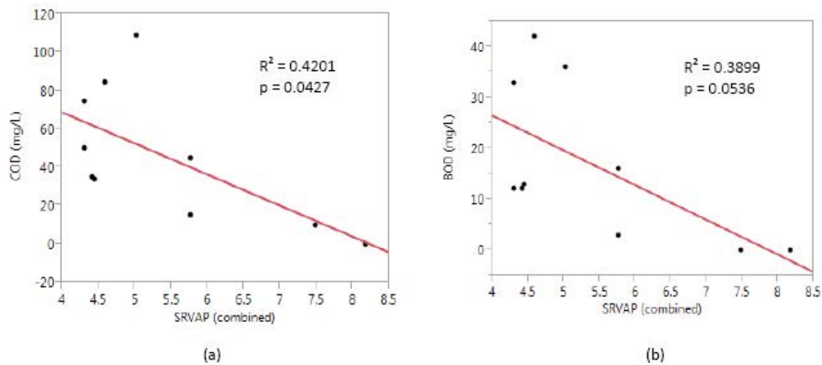
Figure 3: Correlation of SRVAP with (a) COD and (b) BOD.
