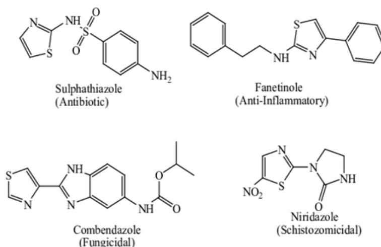
Figure 10. Thiazoles with substitutes showing various activity.
