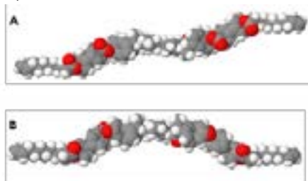
Figure 1: (A) Trans-Conformation of odd spaced dimer (B) Cis-Conformation of even spacer dimer
