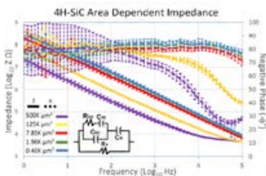
Figure 1. Electrochemical impedance spectroscopy (EIS) performed on all-SiC electrodes of varying geometrical surface areas. Error bars represent standard deviation. Inset shows basic circuit model which produced an impedance profile similar to those obtained experimentally.
