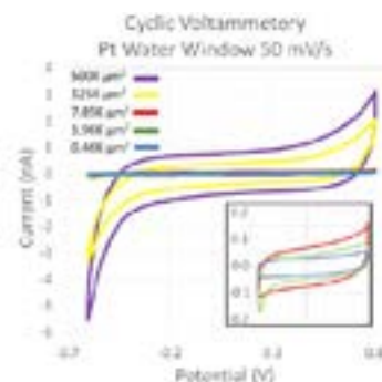
Figure 2. CV plot showing single cyclic voltammetry sweep a select all-SiC electrode. Sweep bounded by potentials typically used for platinum or iridium electrodes of -0.6 V and 0.8 V. Inset shows detail for the three smallest electrodes. All tests performed in naturally aerated PBS (i.e., no of gas bubbling) of 7.4 pH.
